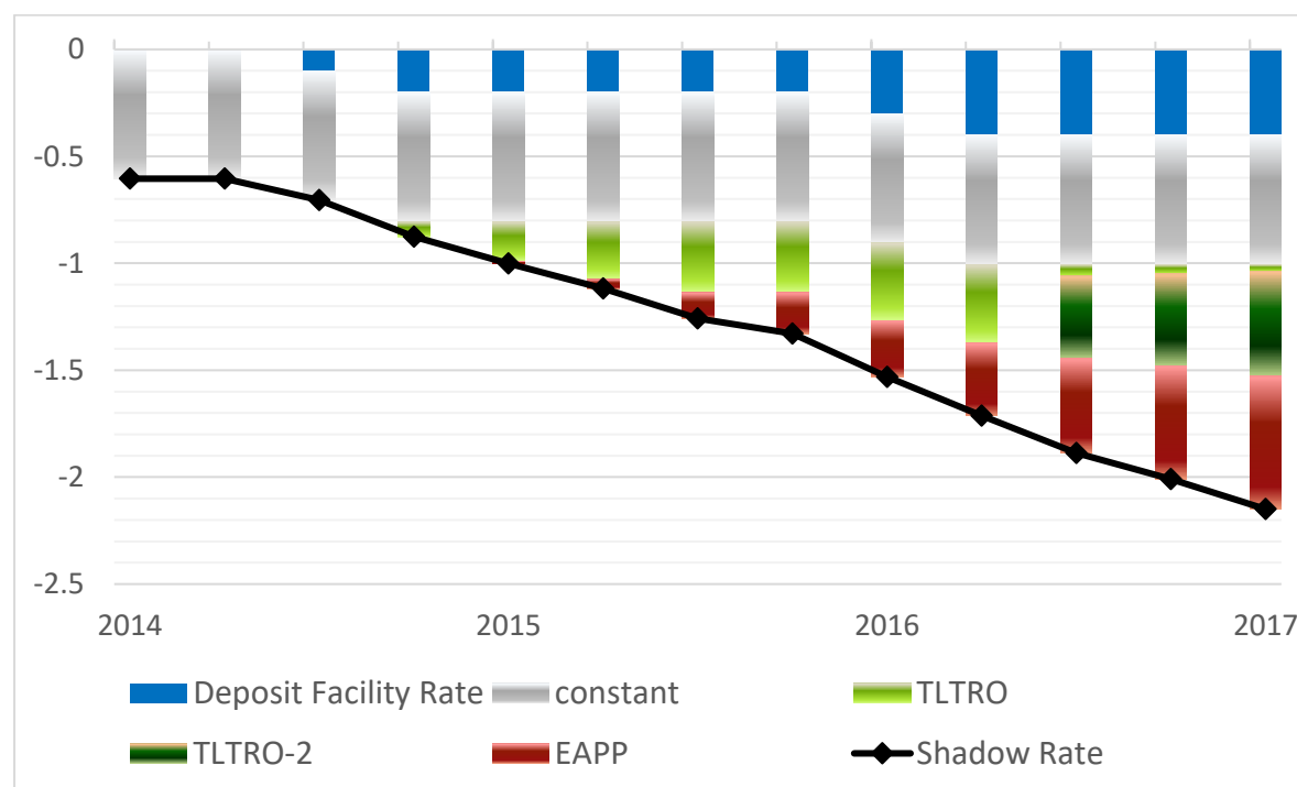
Figure 11. Decomposition of the negative shadow rate.
